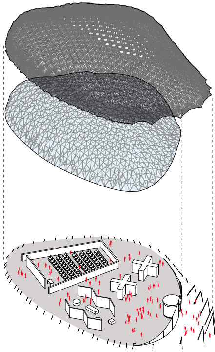
Exploded view - SD Pavilion
